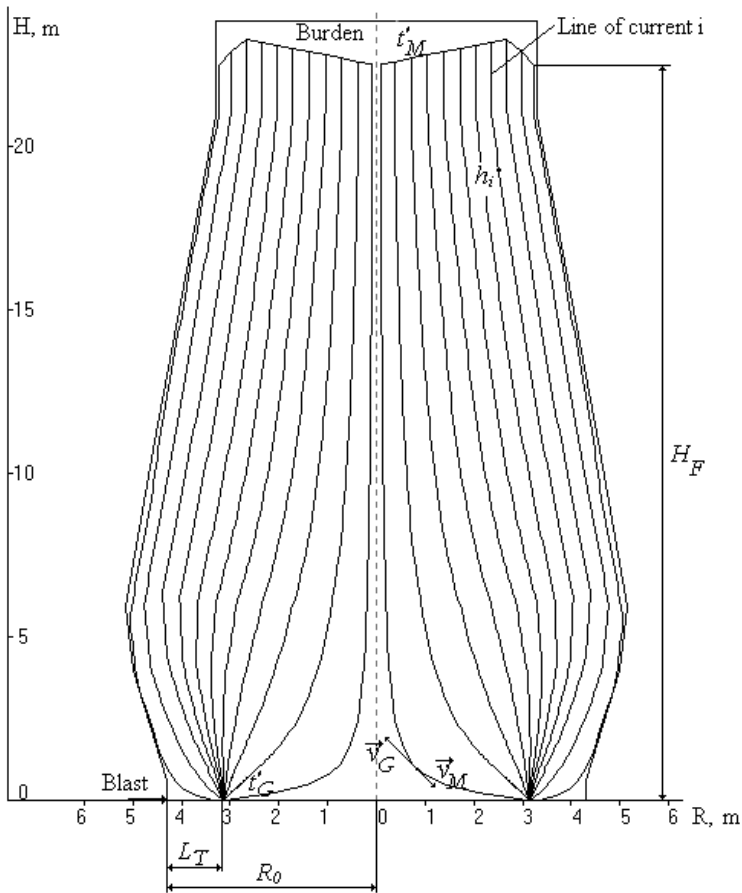
Figure 2.1: To the formulation of the problem of constructing a mathematical model of the blast furnace process: H_F and R_0 are the height of the charge layer and the radius of the furnace, respectively; L_T is the distance from the furnace wall to the center of the tuyere chamber; \vec{v}_M and \vec{v}_G are the velocity vectors of material (burden) and gas, respectively; t'_M и t'_G are the temperatures of charge and gas, respectively at the entrance to the bed; and h_i is the distance from the level of the charging to the calculated point along the line of current i
