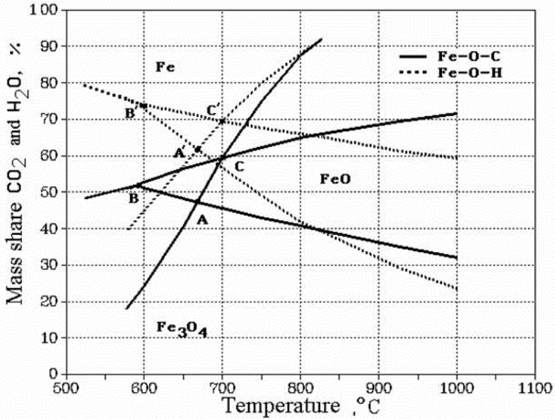
Figure 2.3: The equilibrium diagram of Fe-O-C and Fe-O-H.
