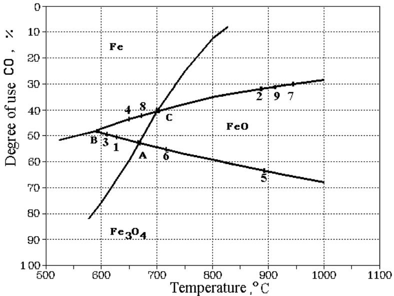
Figure 1.1: Equilibrium degrees of gas use, taken in calculating the minimum coke consumption (for the number of points, see Table 1.1)
