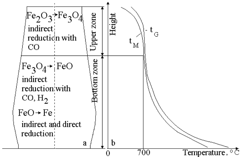
Figure 2.2: Scheme of division of a blast furnace into zones (a) and temperature distribution of charge and gas in height (b).
